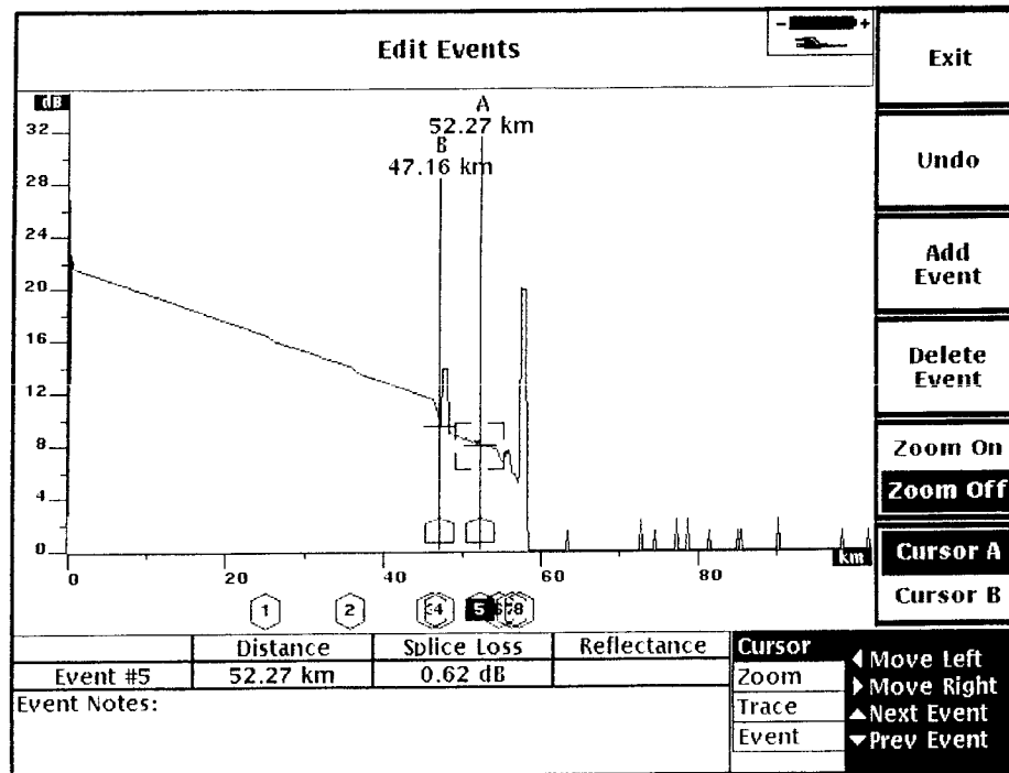
Figure 2–8: Typical User-Placed Event Screen. A New Event (5) is Added at the Location of Cursor A.
