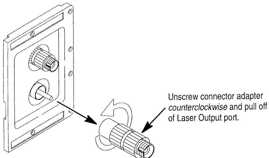
Figure 4–1: Exposing the Laser Output port for Cleaning
