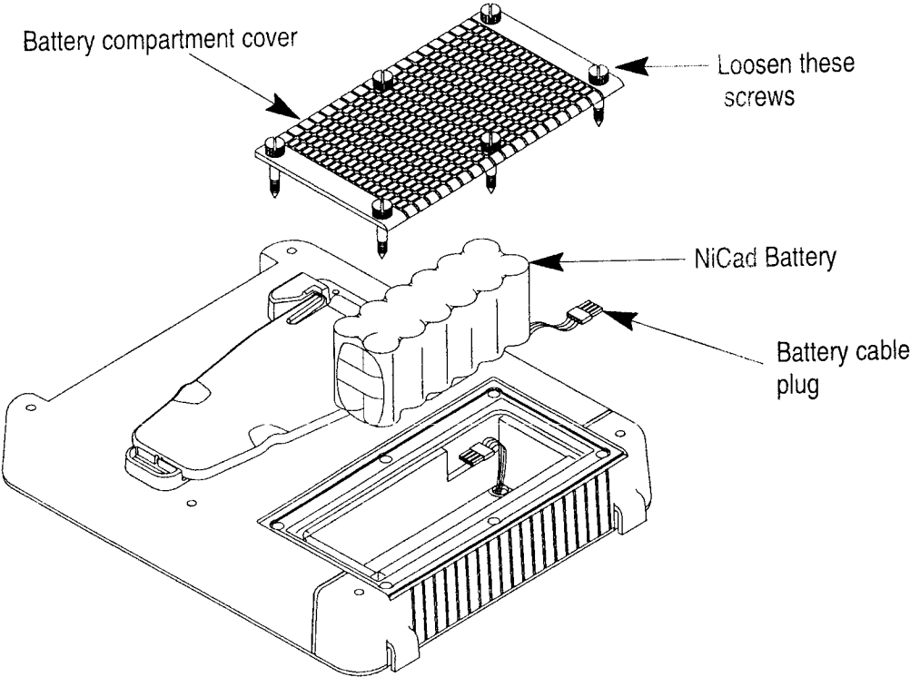
Figure 3-2: NiCad Battery Disconnection, Removal and Replacement
