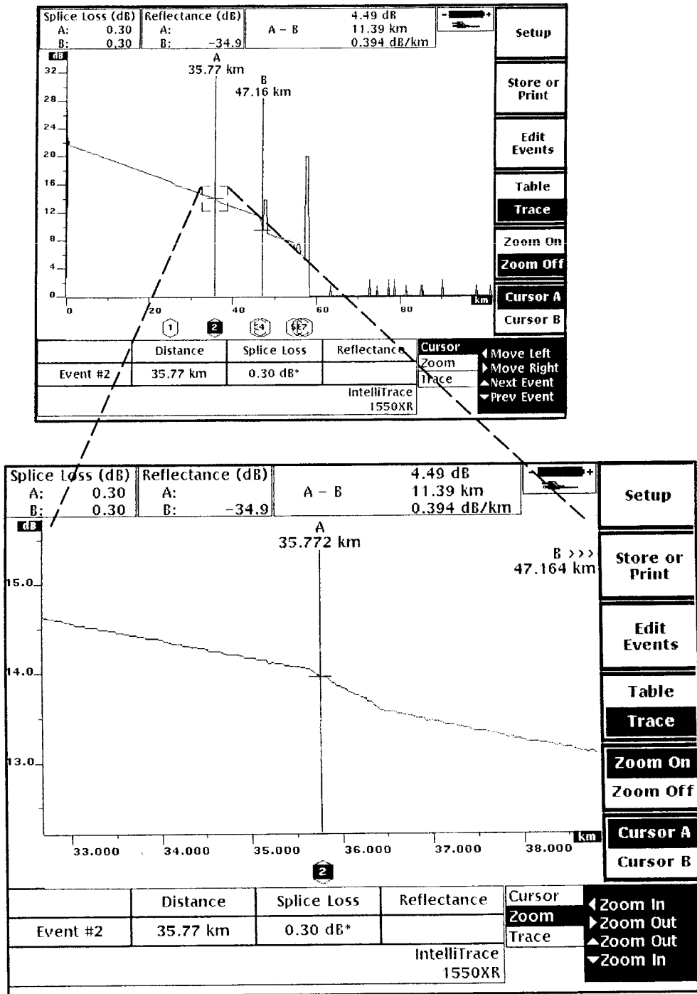
Figure 2-7: Typical Zoomed Waveform Screen. Event 2 is Zoomed.
