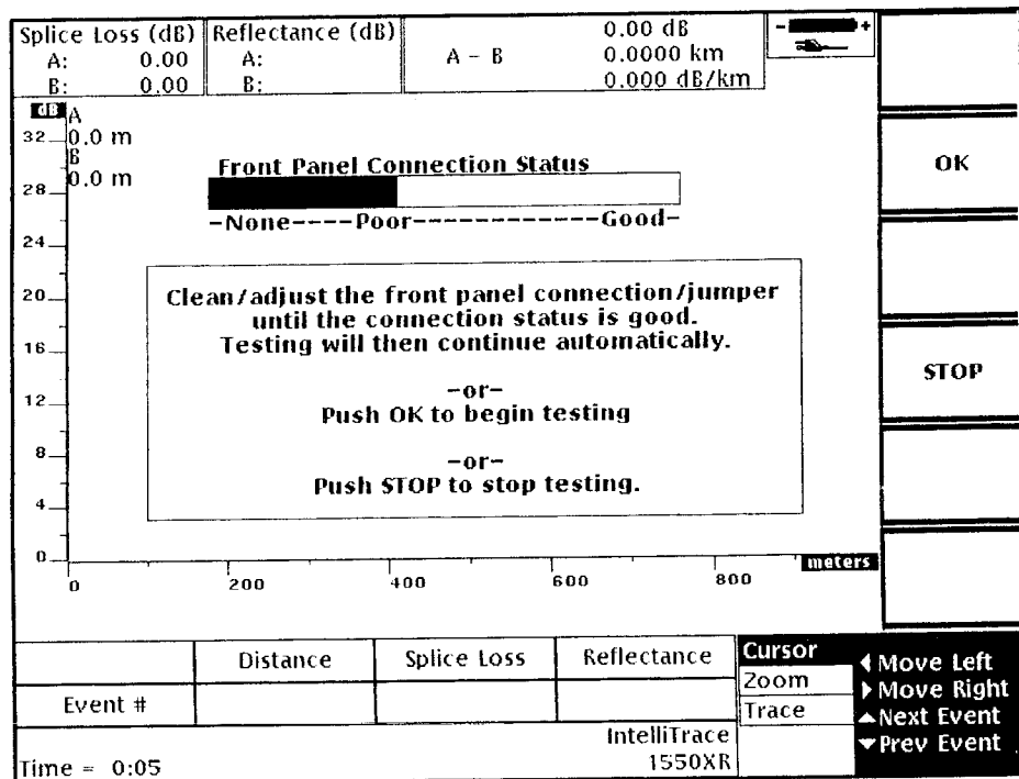
Figure 4-5: Example Front Panel Connection Status Message
