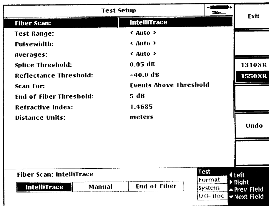
Figure 1–3: Typical Setup Screen.
