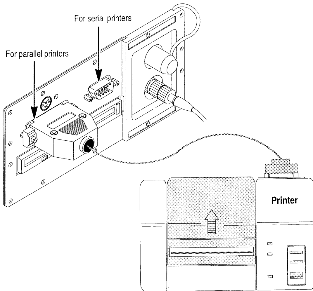
Figure 2-17: Seiko DPU411 Printer Connected to Parallel Port
