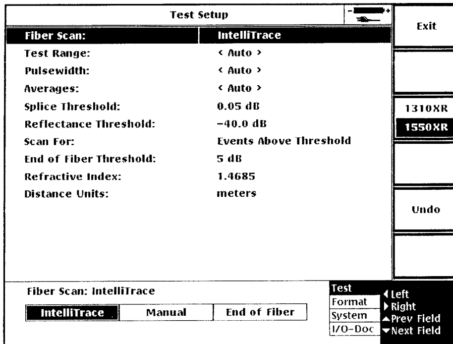
Figure 1-4: Typical Test Setup Menu Screen.
