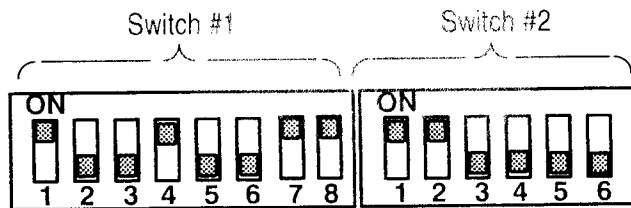
Seiko DPU411 Switch Settings for Parallel Interface
