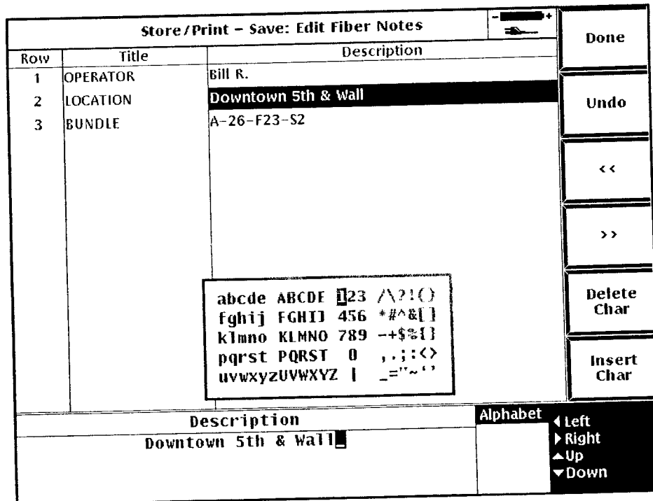
Figure 2-13: Editing a Fiber-Note Field.
