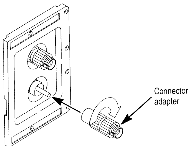
Figure 1–1: Connector Adapter Installation
