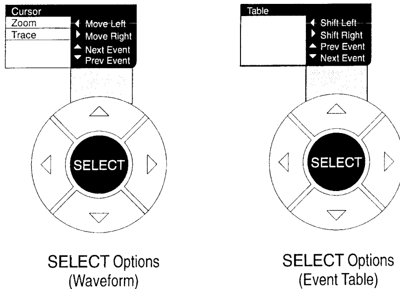
Figure 2-6: SELECT Button Options
