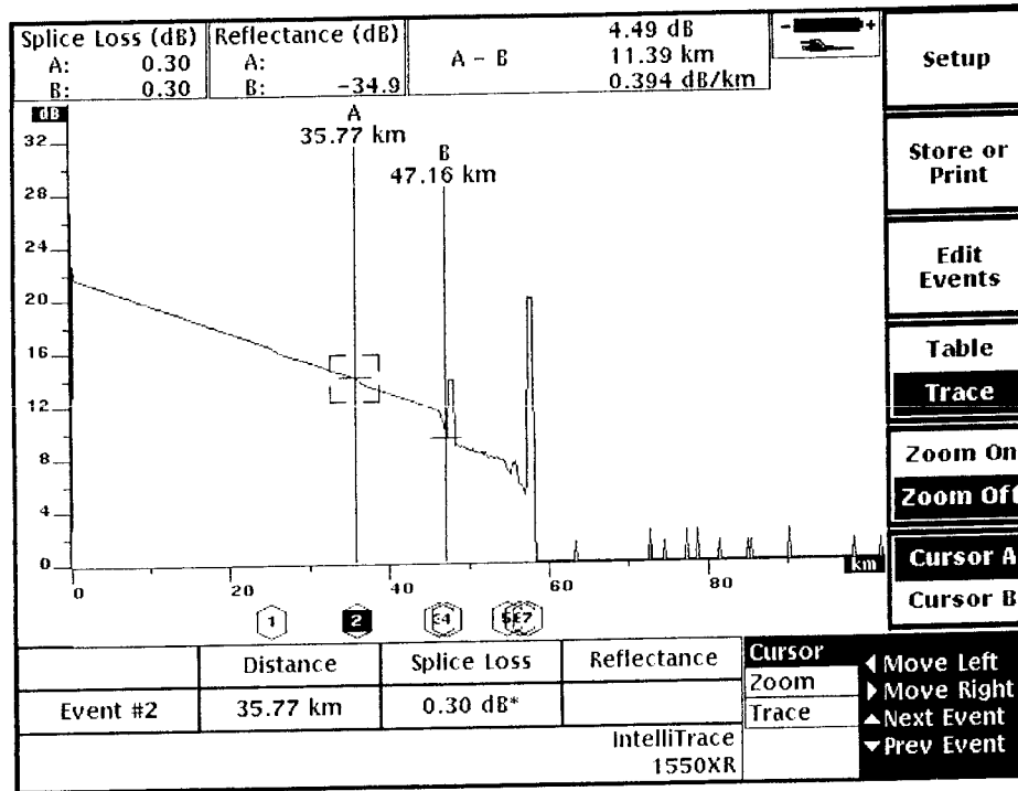
Figure 2–2: Typical Waveform Screen. Event 2 is Selected.
